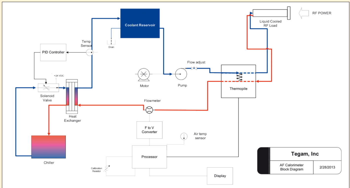
Figure 1: Block diagram of the calorimeter used as the starting point for this project
